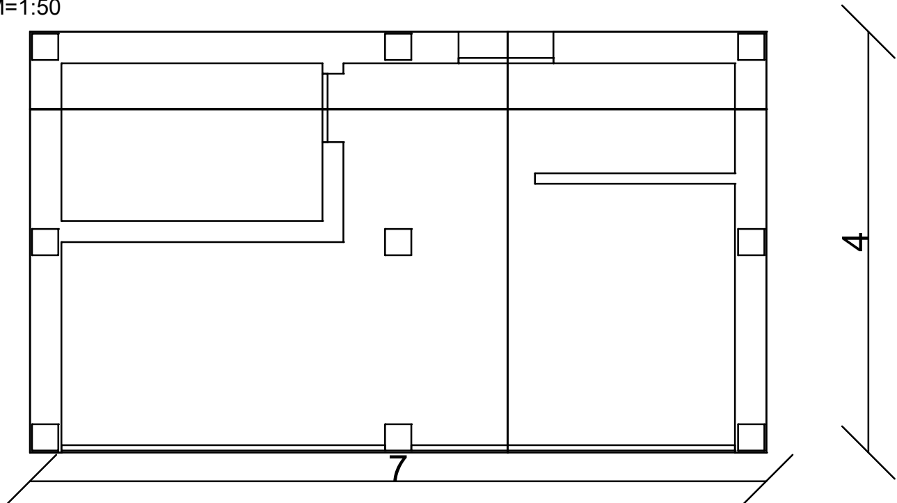
floorplan M=1:50
