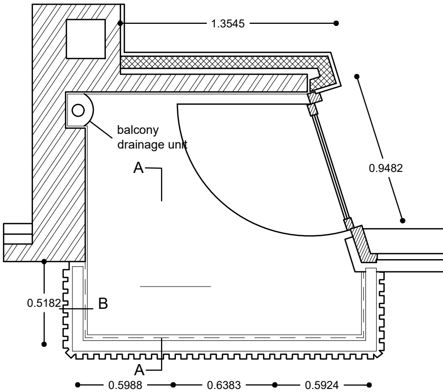
KEY PLAN OF BALCONY scale 1/24
