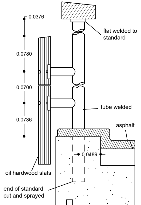
1/4 FULL SIZE DETAIL AT 'B'
