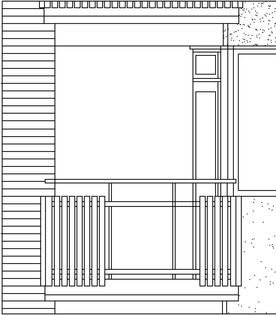
ELEVATION OF BALCONY scale 1/24
