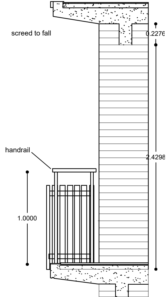
SECTION A-A scale 1/24
