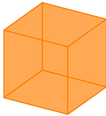
HEXAEDRO
