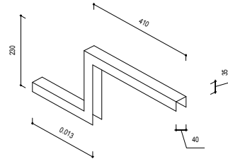
ISOMETRICS OF MS BRACKET
