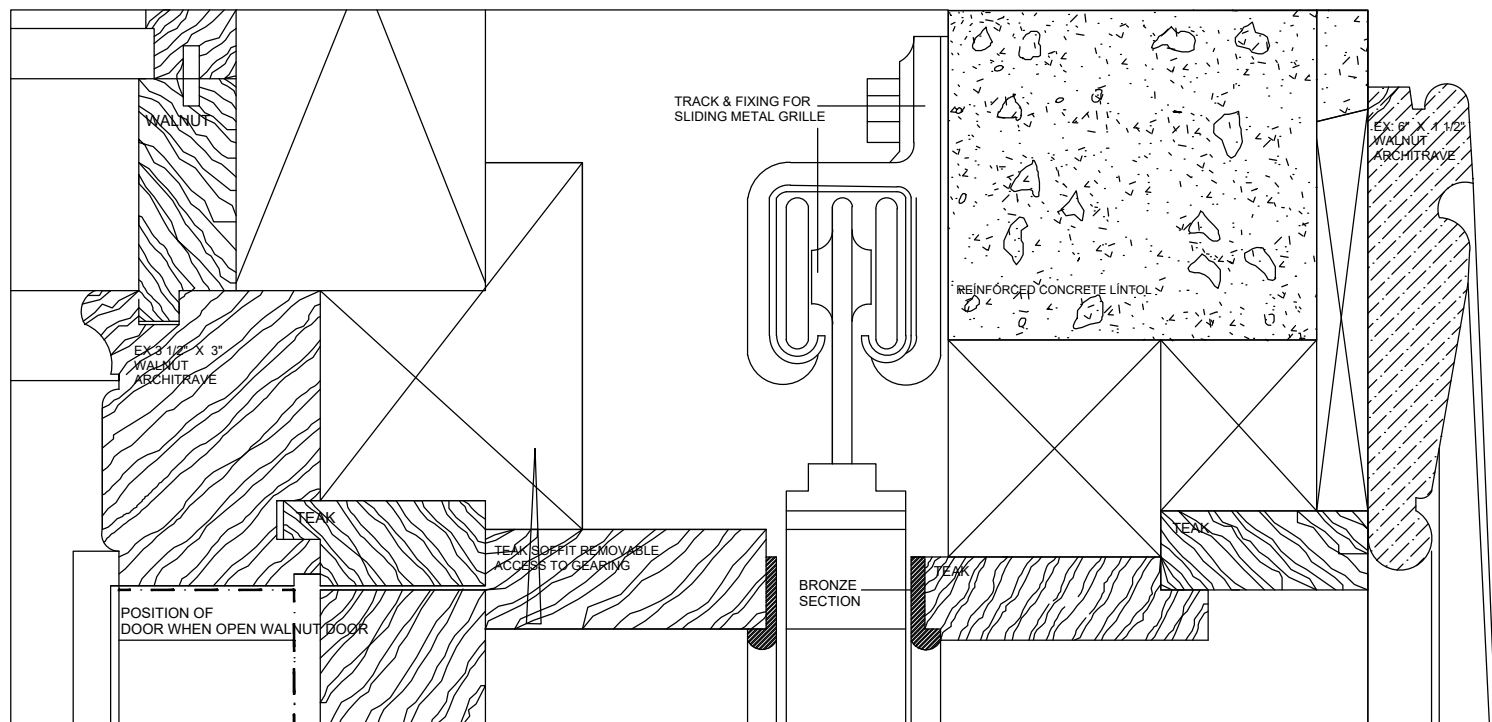
DETAIL SECTION THRO' HEAD OF DOORS & GRILLE
