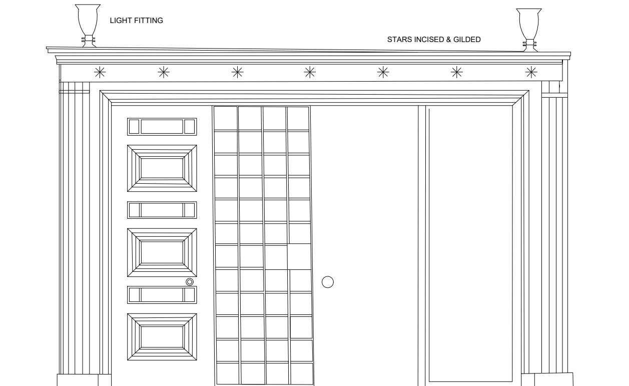
ELEVATION WITH DOOR OPEN SHOWING GRILLE
