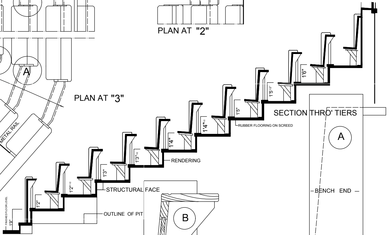
OUTLINE OF PIT
