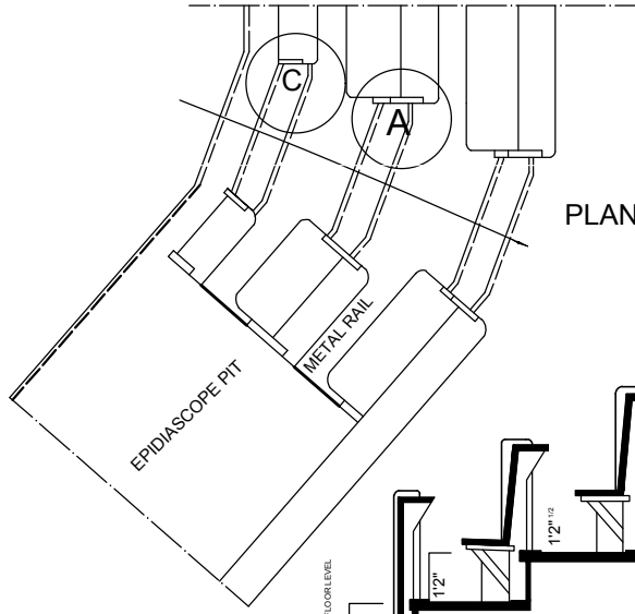
PLAN AT "1"
