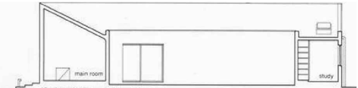
North-south section; scale: 1/150.
