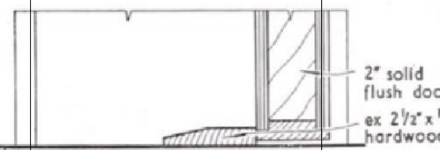
THRESHOLD DETAILS OF DOOR. scale \frac{1}{4} full size
