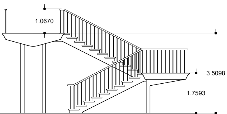
CROSS SECTION THRO' STAIR. (A-A). scale 1:4
