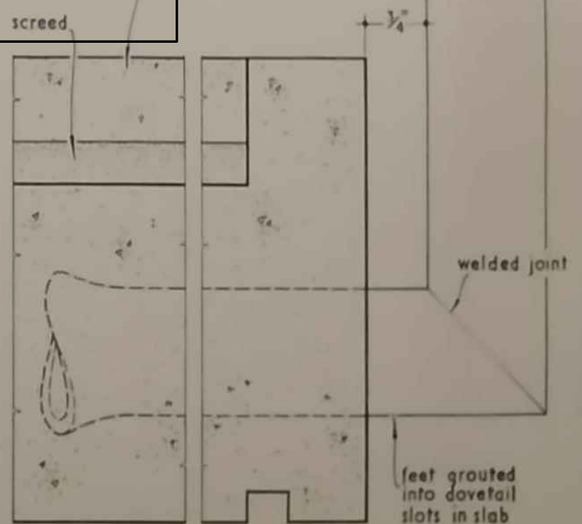
SECTION THRO' BALUSTRADE. scale \frac{1}{2} full size
