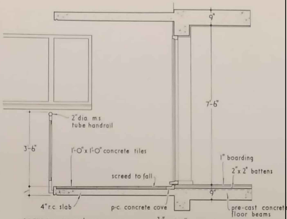
SECTION THRO' BALCONY. scale \frac{3}{8}'' = 1'-0''
