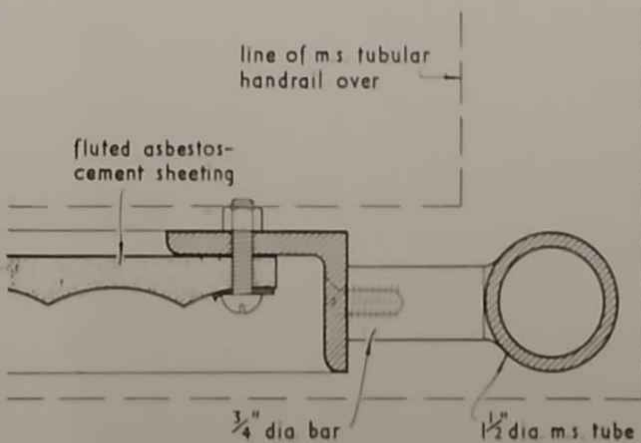
PLAN AT A scale \frac{1}{2} full size
