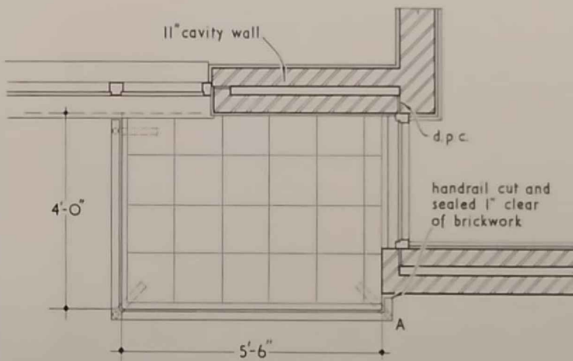
PLAN OF BALCONY. scale \frac{3}{8}'' = 1'-0''
