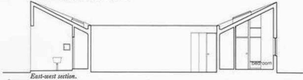
East-west section.
