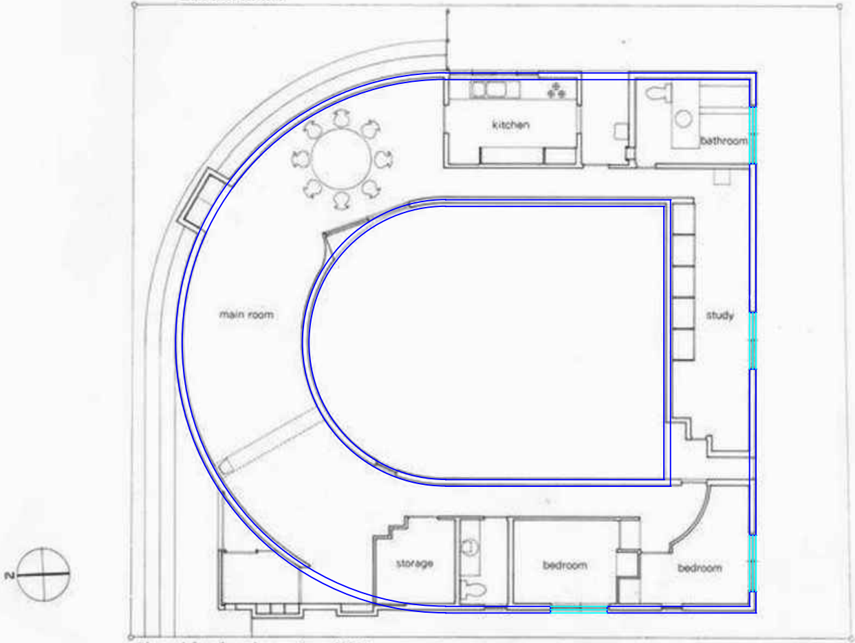
Plot and first-floor plan; scale: 1/150.
