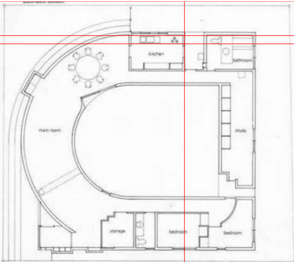
Plot and first-floor plan; scale: 1/150.
