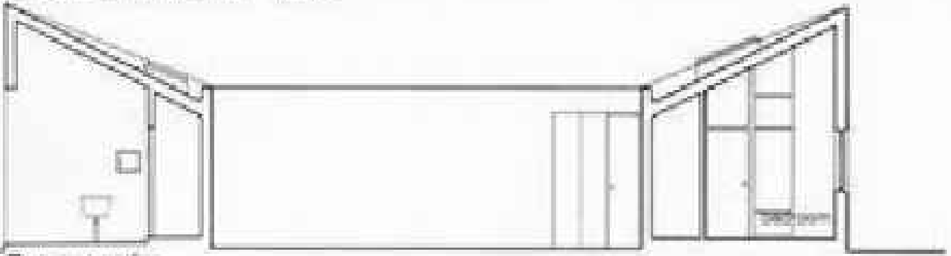
East-west section.
