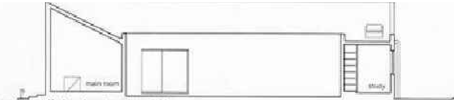
North-south section; scale: 1/150.
