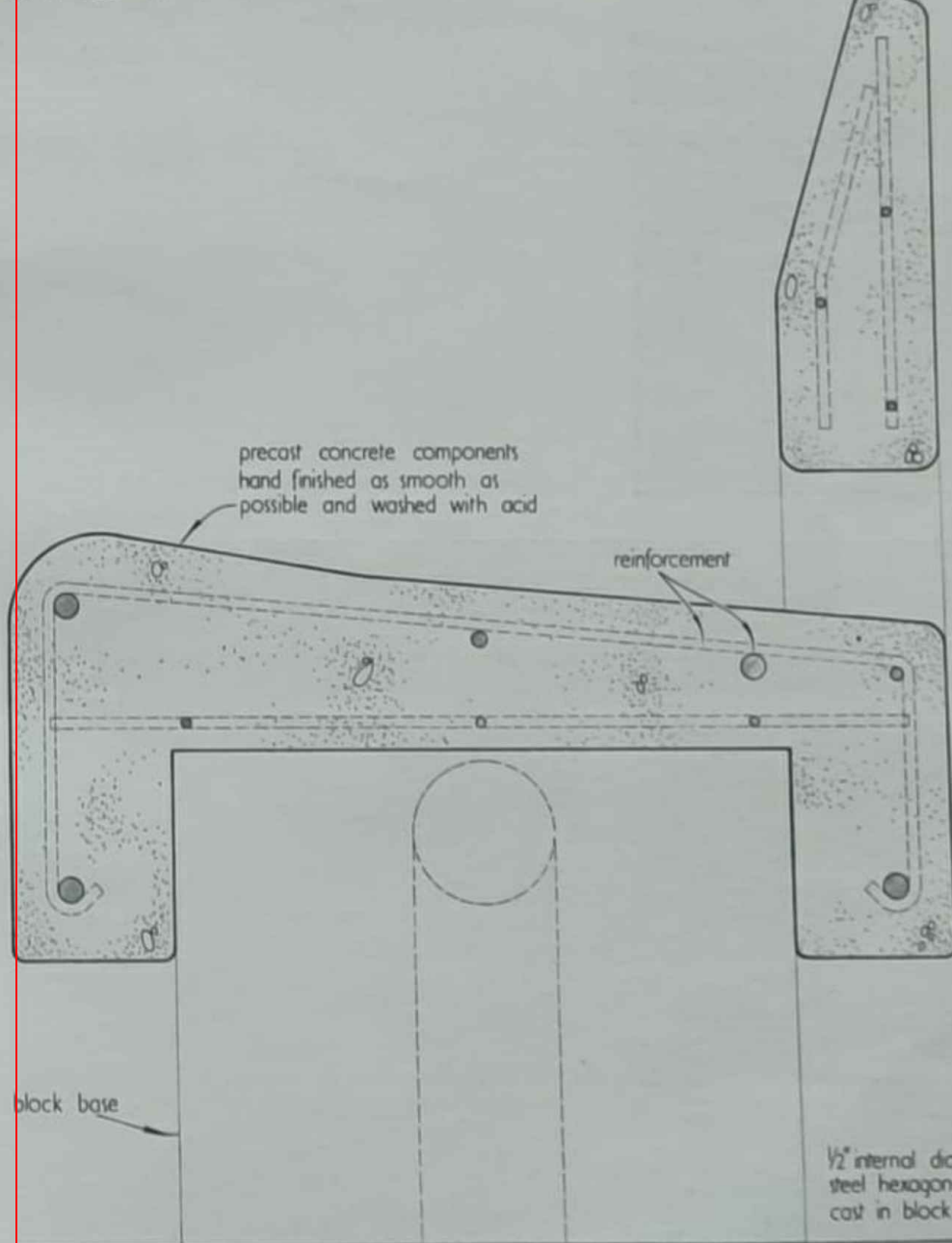
SECTION A-A scale 1/4 full size
