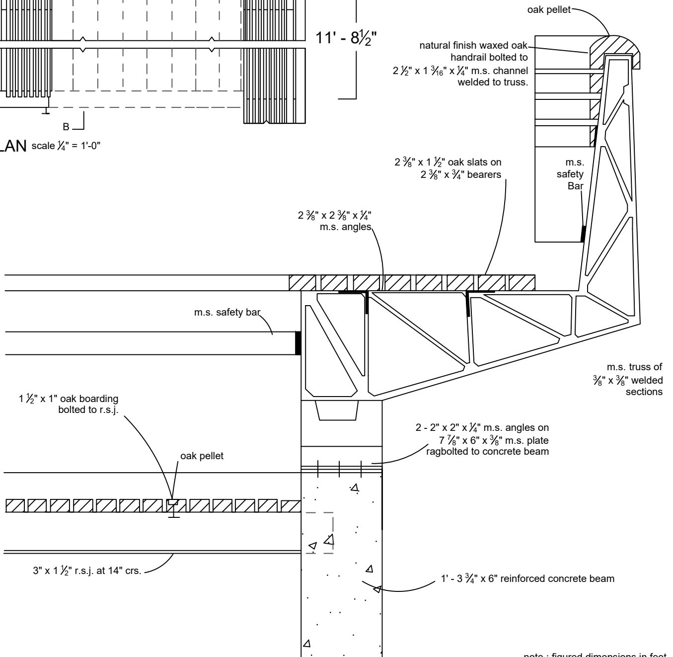
DETAIL SECTION scale 1/8 full size
