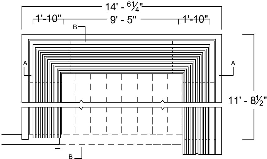
PLAN scale 1/4"=1'-0"
