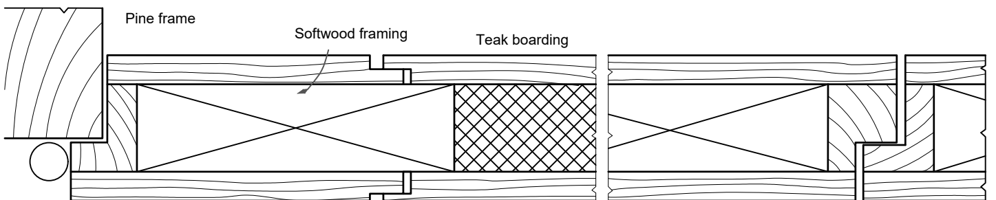
HORIZONTAL SECTION. Scale 1/2
