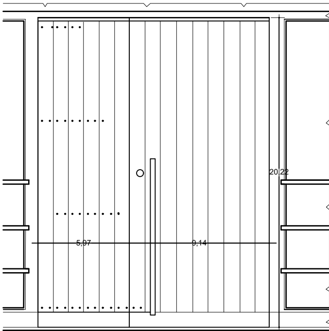
ELEVATION. Scale 1/24
