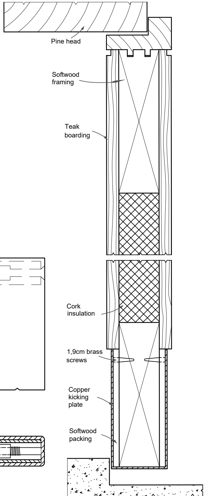
VERTICAL SECTION. Scale 1/2
