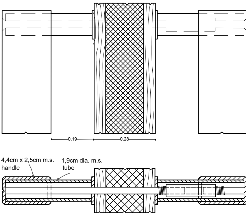
SECTION AND PLAN SHOWING FIXING OF HANDLES. Scale 1/2
