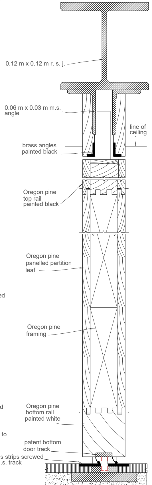
SECTION D - D. scale 1/3
