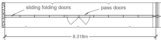
PLAN. scale 1/100
