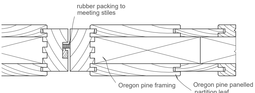
PLAN AT B. scale 1/3
