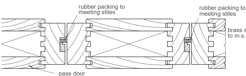
PLAN AT C. scale 1/3
