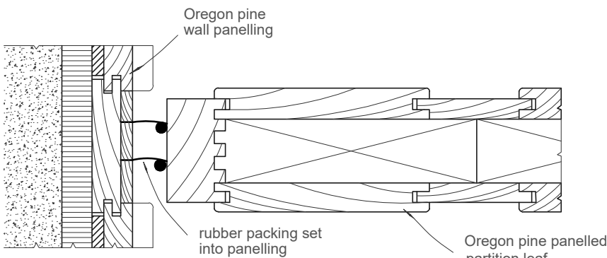
PLAN AT A. scale 1/3
