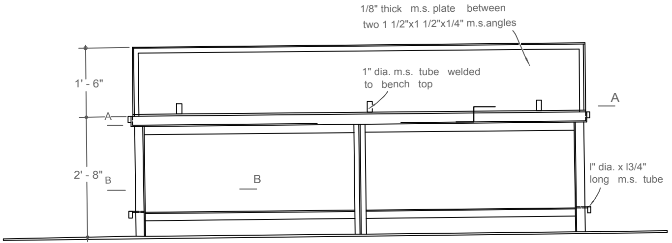
ELEVATION N . scale 1/2" = 1' - 0"
