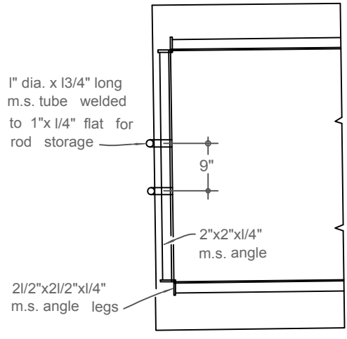
PLAN AT B - B. scale 1/2" = 1' - 0"
