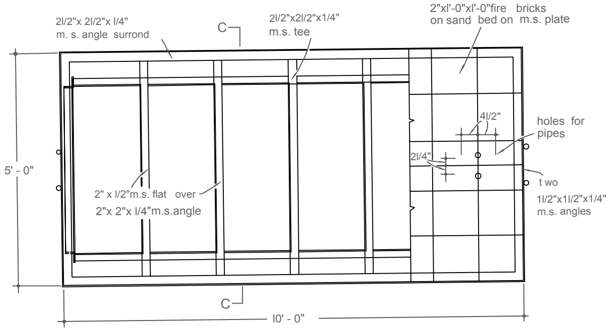
PLAN AT A - A. scale 1/2" = 1' - 0"
