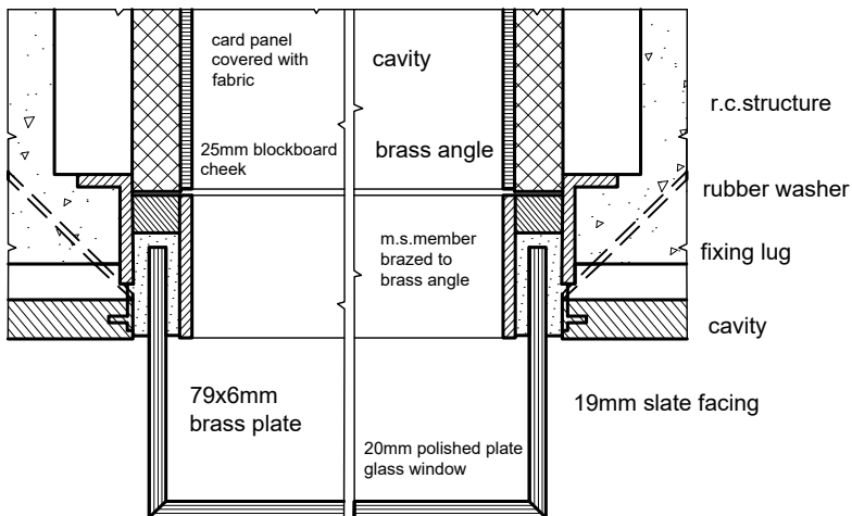
PLAN scale 1:4
