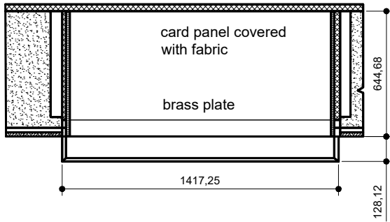
PLAN scale 1:30
